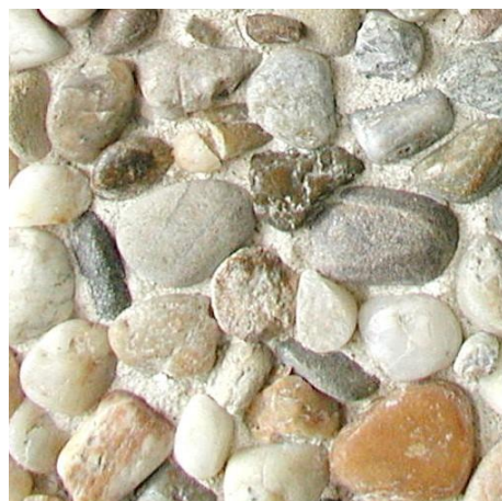
74 Washed concrete Danube gravel 11/16mm BC
